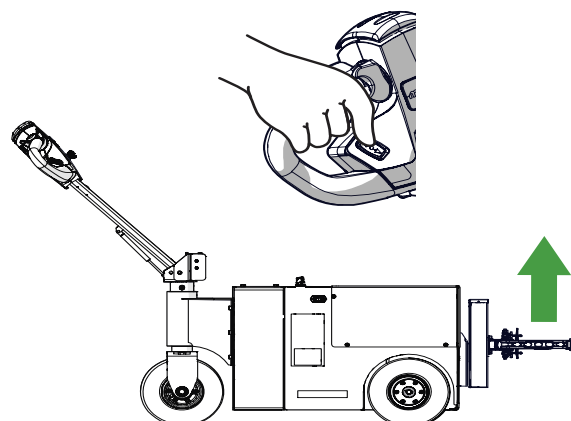
Figure 11. Raising the hook
