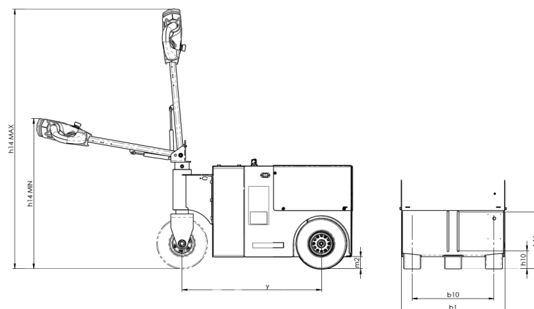
Figure 18. Product dimensions (side view)
