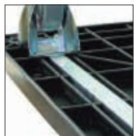
Fitted with steel reinforcing bars to underneath of platform
