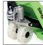
Sealed hydraulic pump with nylon steering wheels
