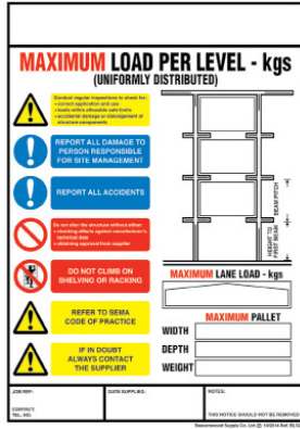
Drive-in racking
