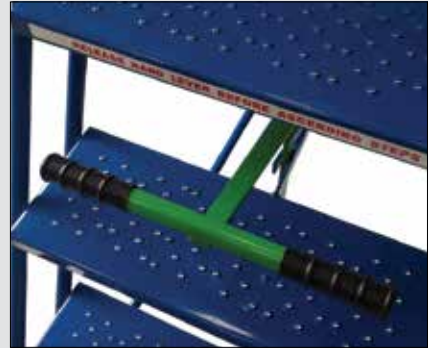
'Access barred' central lever brake
